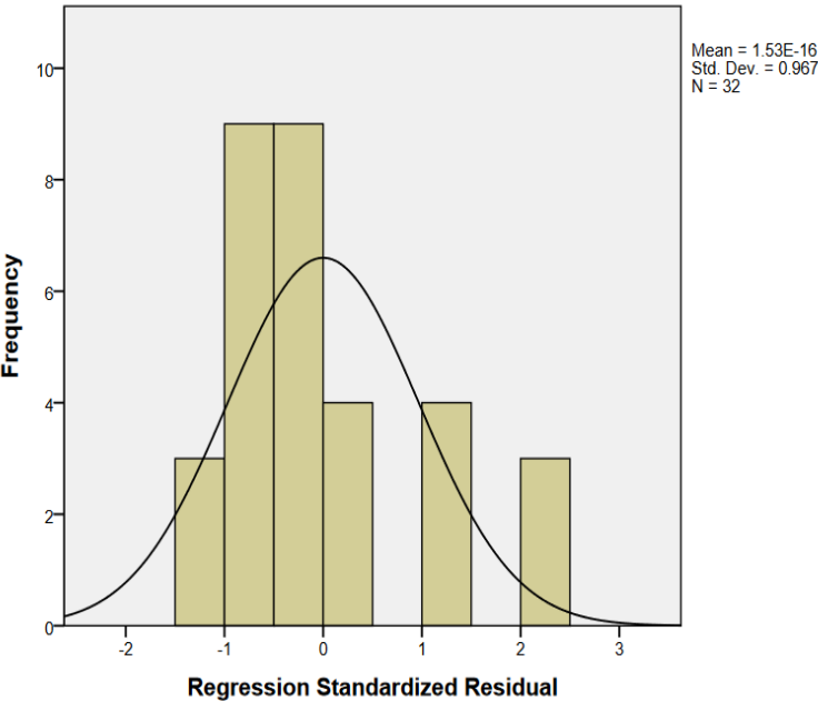
Gambar 1. Histogram
